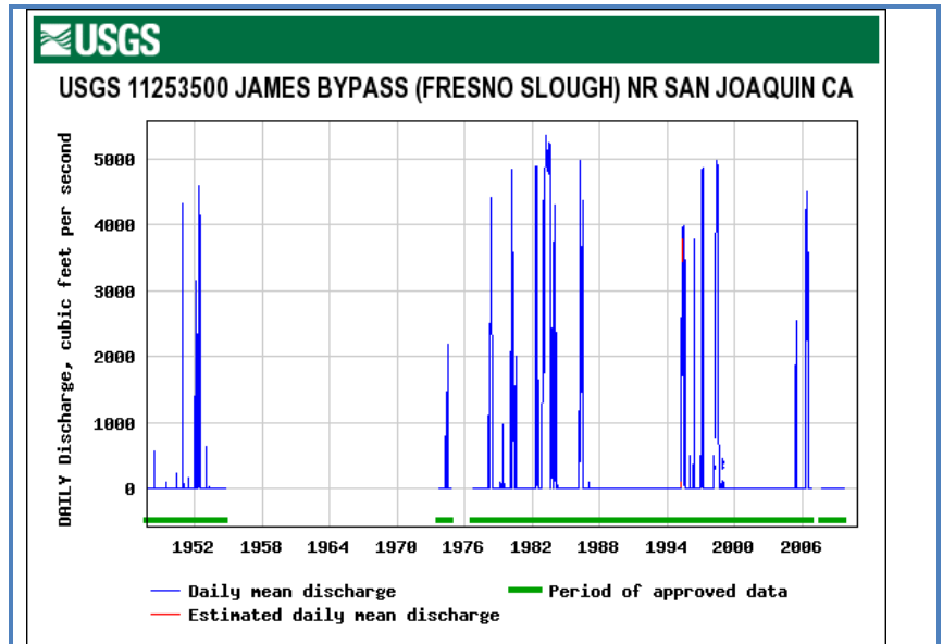
Figure 1. Flood flows past the James Weir have a reoccurrence interval of 2 – 3 years and vary greatly in magnitude, at times exceeding 4750 CFS system design.
